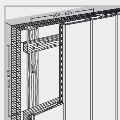
2. Vertical installation (selekta)
