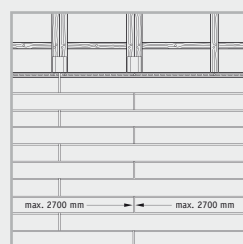
3. Horizontal installation in staggered arrangement (selekta)
